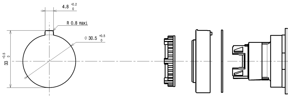
BACO super flush buttons requires a specific 30 mm cut out on the panel to be mounted.
